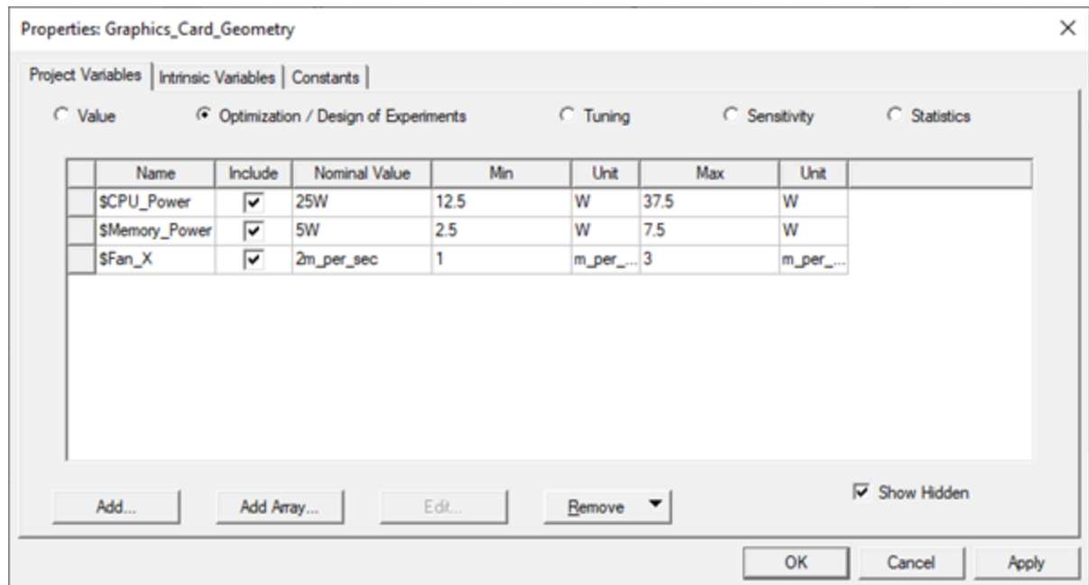
Figure 6-2: Properties dialog box with variables
